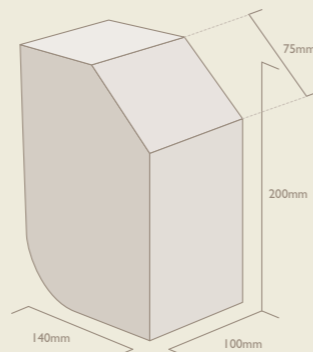
Q Kerb High Chamfered Position
