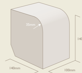
B Kerb Bullnose Position
