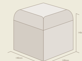
B Kerb Small External Bullnose Corner
