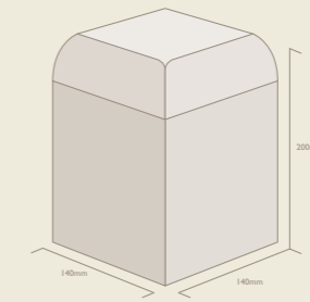
Q Kerb High External Bullnose Corner
